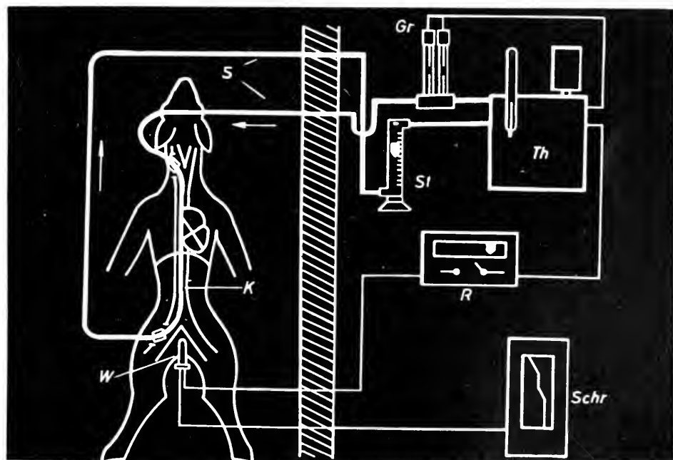
FIG. 1.—Diagram of Kerckhoff Institut hypothermia preparation using intravascular brine cooling of blood.
